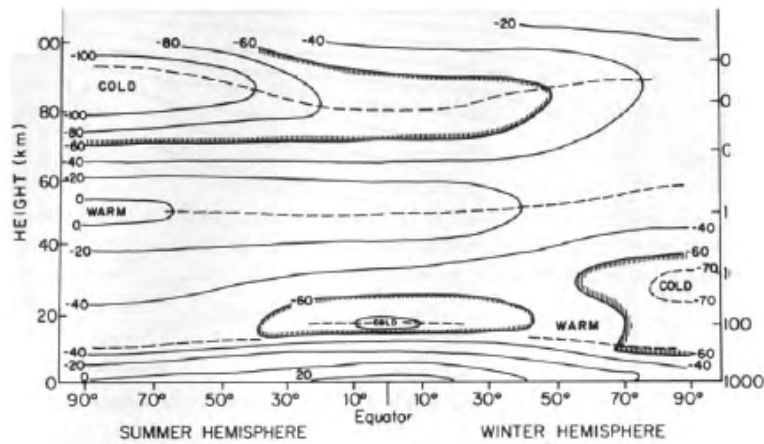
Fig. 1.3. Schematic latitude-height section of zonal mean temperatures (°C) for solstice conditions. Dashed lines indicate tropopause, stratopause, and mesopause levels. (Courtesy of R. J. Reed.)
