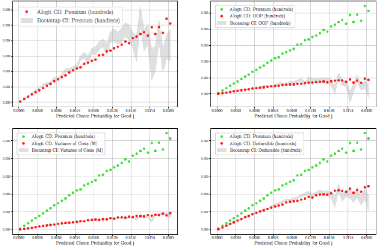
Figure 3: Empirical vs. Model Predicted Cross-derivatives
